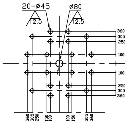
EJECTOR HOLE POSITION
